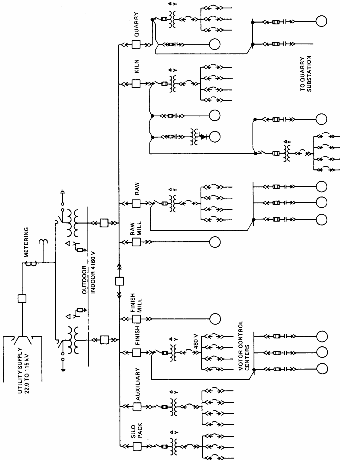
Figure 7—Typical cement plant distribution system
