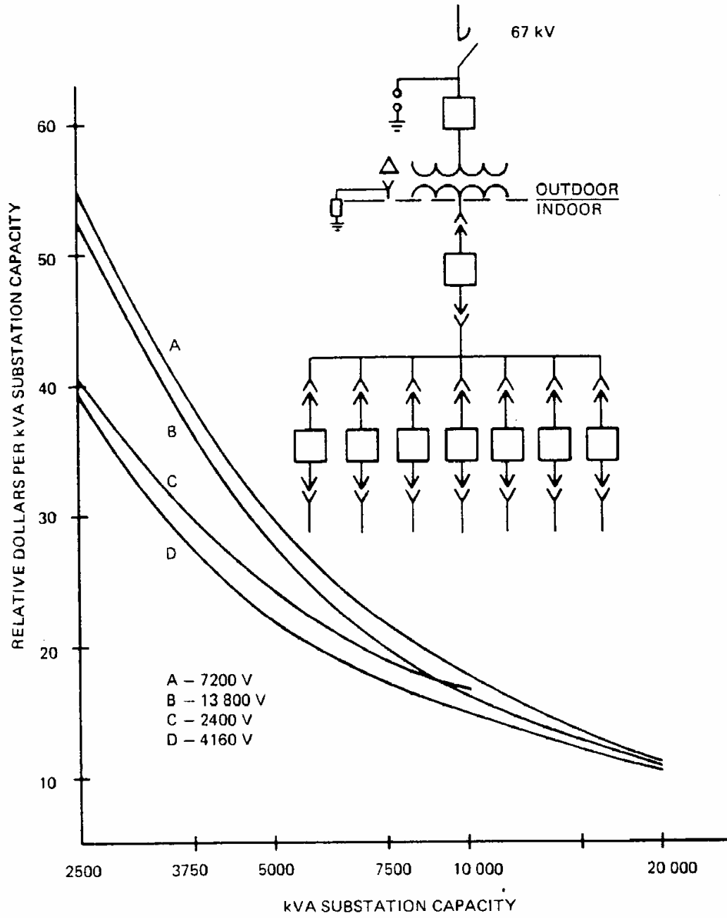
Figure 2—Economic comparison of single-ended substations
