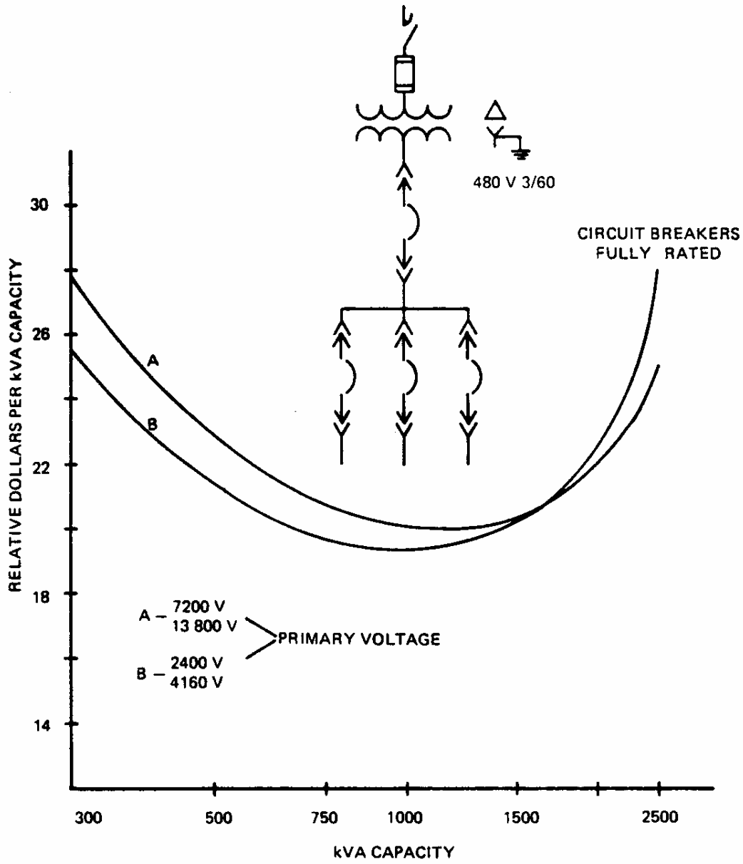
Figure 4—Economic comparison of indoor secondary unit substation
