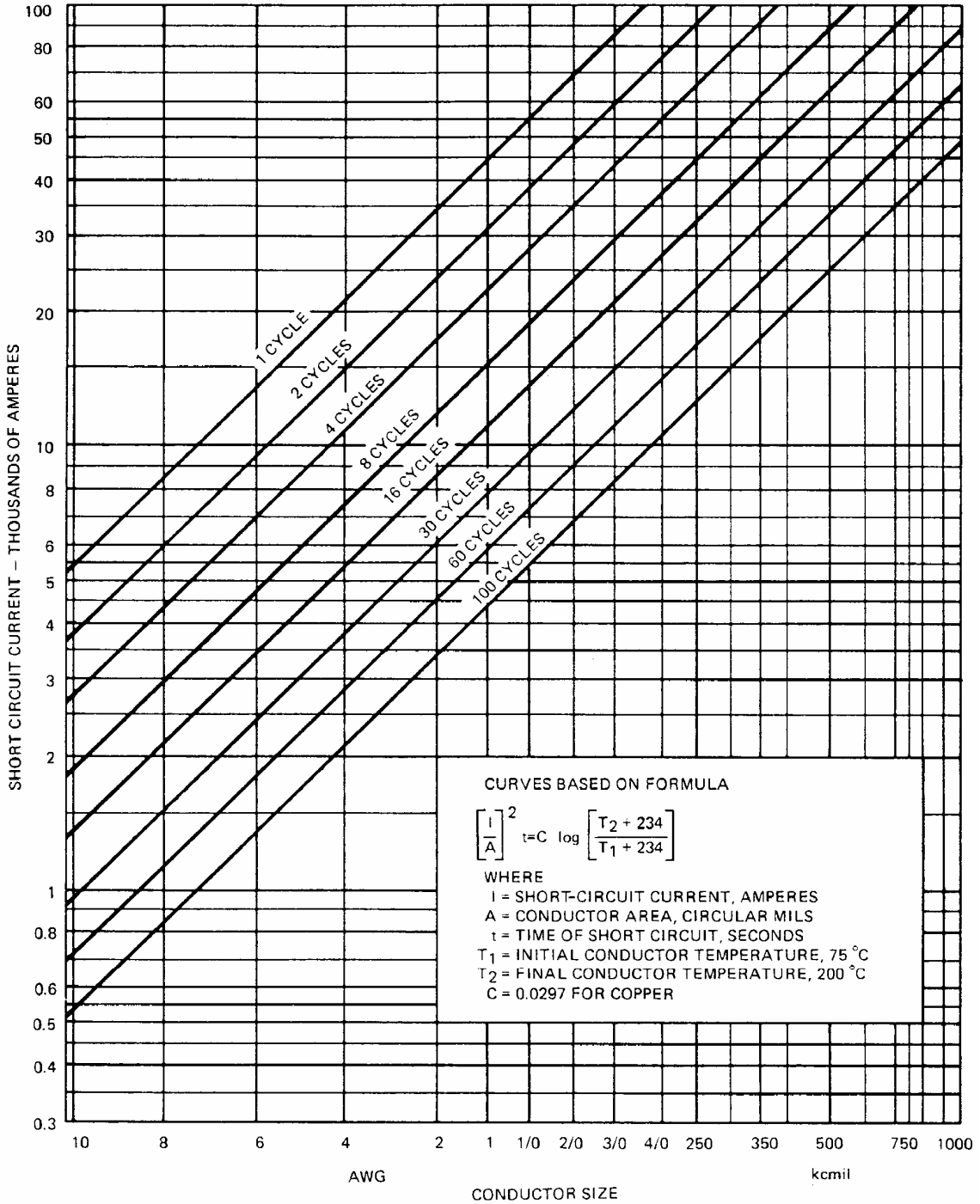
Figure 8—Maximum allowable short-circuit current copper conductor
