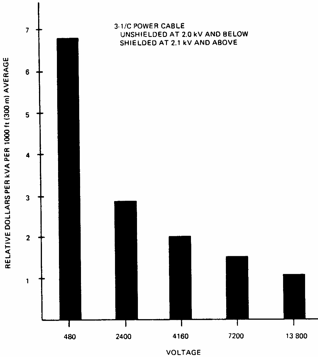
Figure 3—Economic comparison of cable
