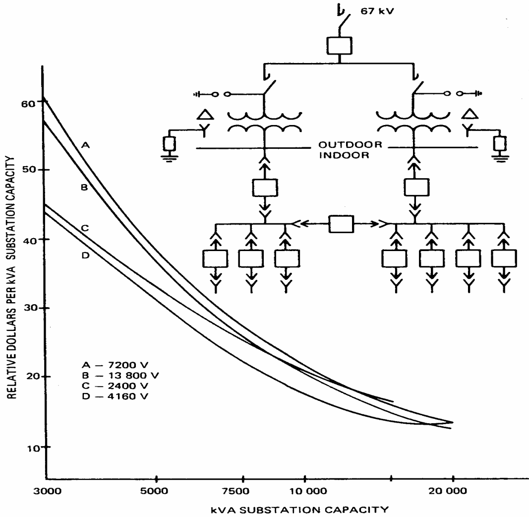
Figure 1—Economic comparison of double substations
